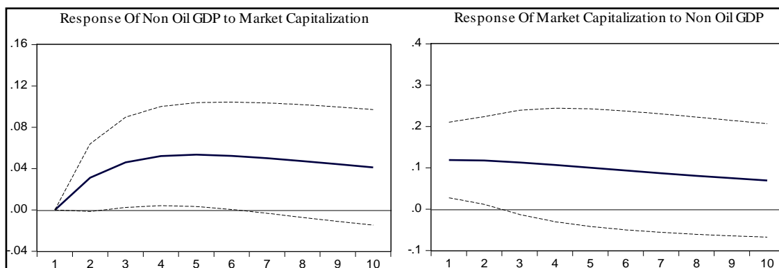
Figure 2. Response Funtcions of the non Oil GDP and Market Capitalization
