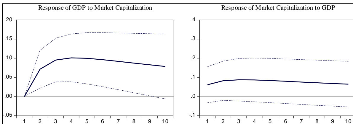
Figure 1. Response Funtcions of the total GDP and Market Capitalization
